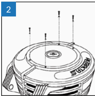
2. Remove screws.
