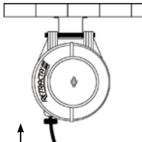
Fig.2 Overhead mounting (max height 4.5m / 14.7ft)
